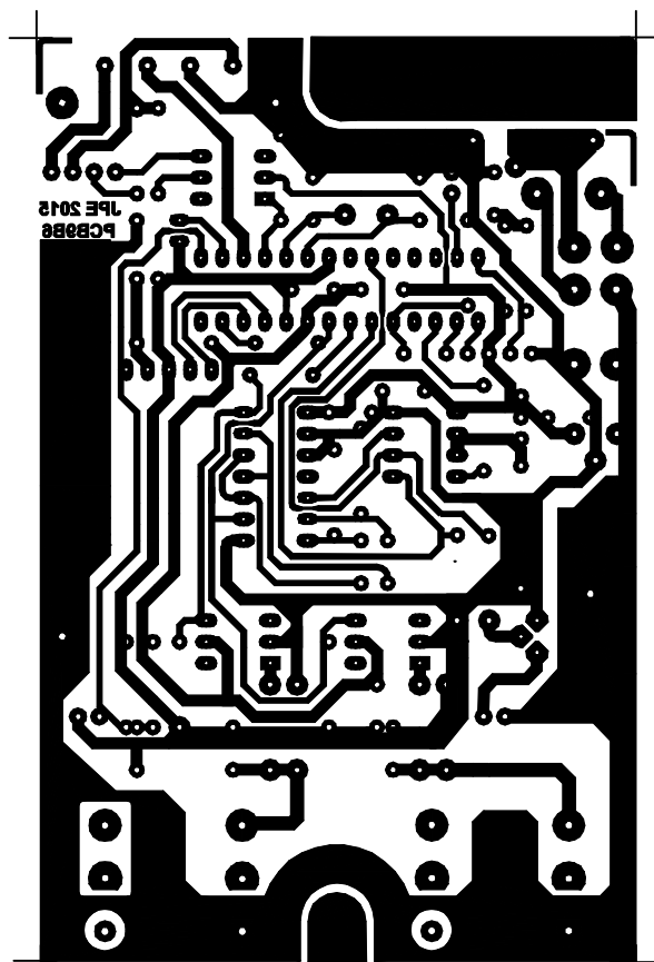
PCB Print Layout
